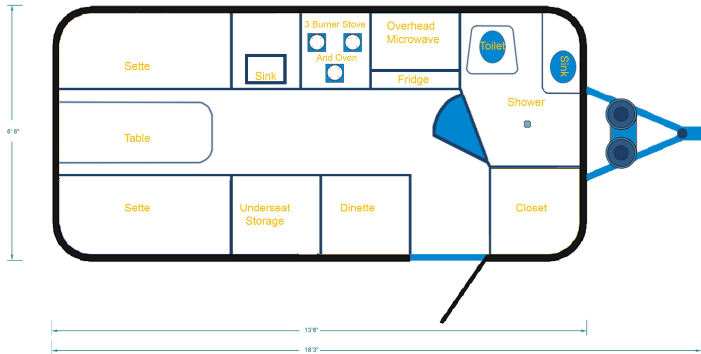
Cortes 18BK DAY FLOOR PLAN Sleeps 2-3 (RV King Bed)
